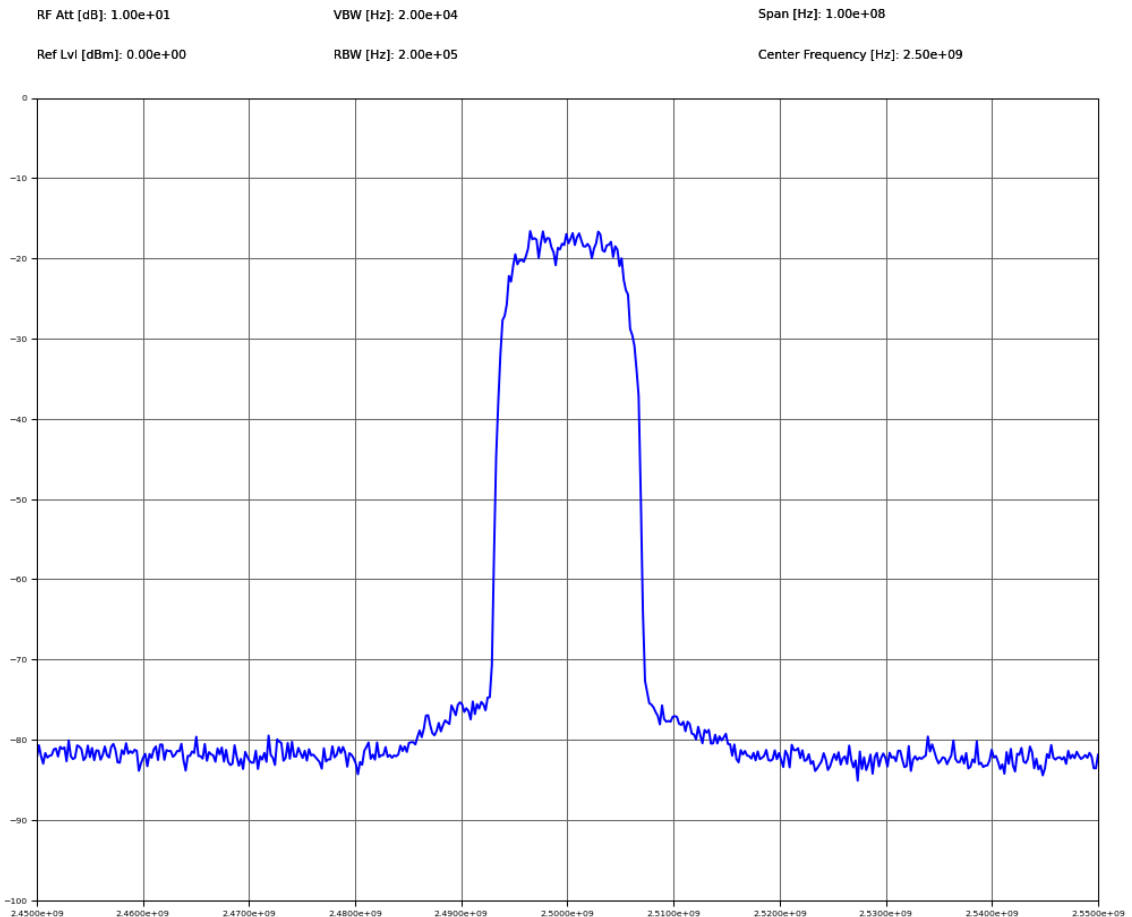
Figure 12: 256QAM 10 MS/s
