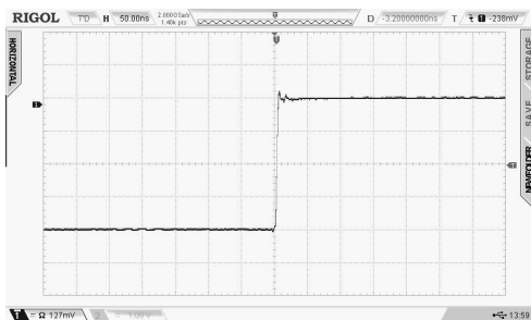
Figure 3 Waveforms Generated without Extending the Input Cable
