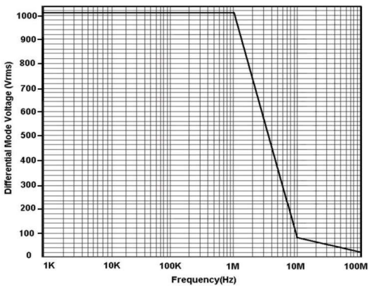
Figure 5 PHA0150/PHA1150/PHA2150 Max. Differential Mode Voltage vs Freq.
