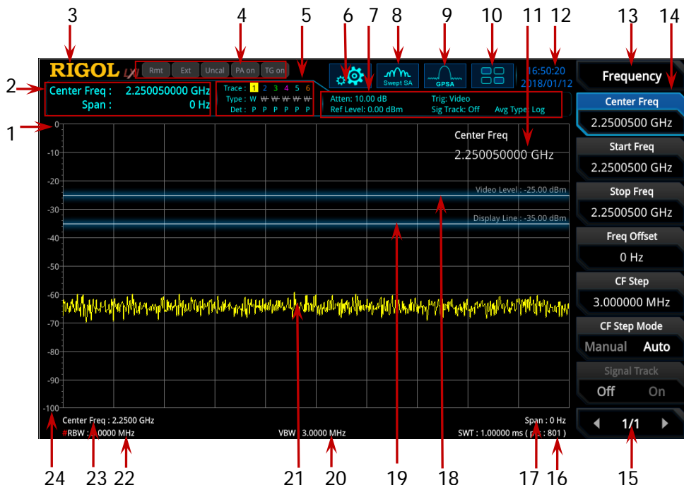
Figure 1-9 User Interface
