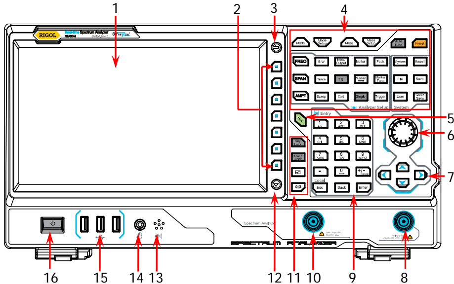
Figure 1-4 Front Panel
